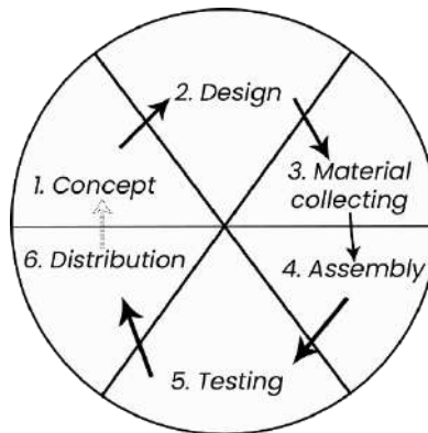
Gambar 1. Metode MDLC
